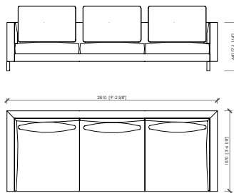
DIVANO 3 POSTI / 3-SEATER SOFA_281X107
