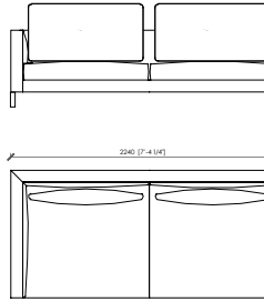
LATERALE DX/SX / SIDE L/R _ 224x107
