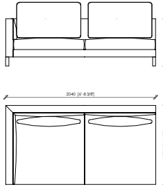
LATERALE DX/SX / SIDE L/R _ 204x107
